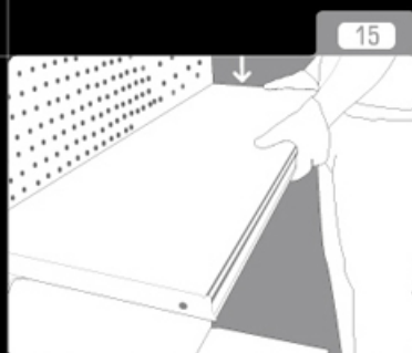
Lift the front of the shelf up until roughly at a 45° angle. Lock the inner side of the panel on the back edge of the shelf onto the outer edge of the handle. Push down and check whether the tenons on the back edge of the shelf have locked into five grooves on the handle.
