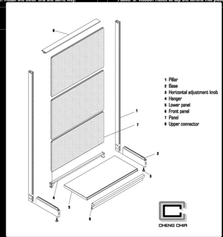
Upper assembly: Push one end of the upper connector into the gap at the end of the pillar until locked into place. Install the other end the same way.
