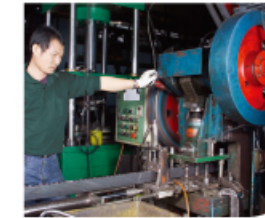
Automatic Punching Machine: full automatic support, with fixed-size compartments between punched holes 20-m compartment with a tolerance within 0.5m/m
