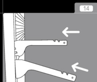
To install handles, push forward into desired holes, and then press down to lock in a horizontal or angled position.
