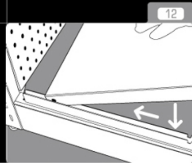
To install the lower panel, hold it by its front edge with both hands and lift up so that the back end faces down. Lock the panels on both ends into the inner groove on the base, push back, and then push down until level.
