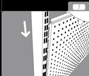
To install panel, put base into position first. Insert the panel into the row of holes in the pillar at one end, and use the same method to lock the other end.
