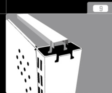
Upper assembly: Push one end of the upper connector into the gap at the end of the pillar until locked into place. Install the other end the same way.
